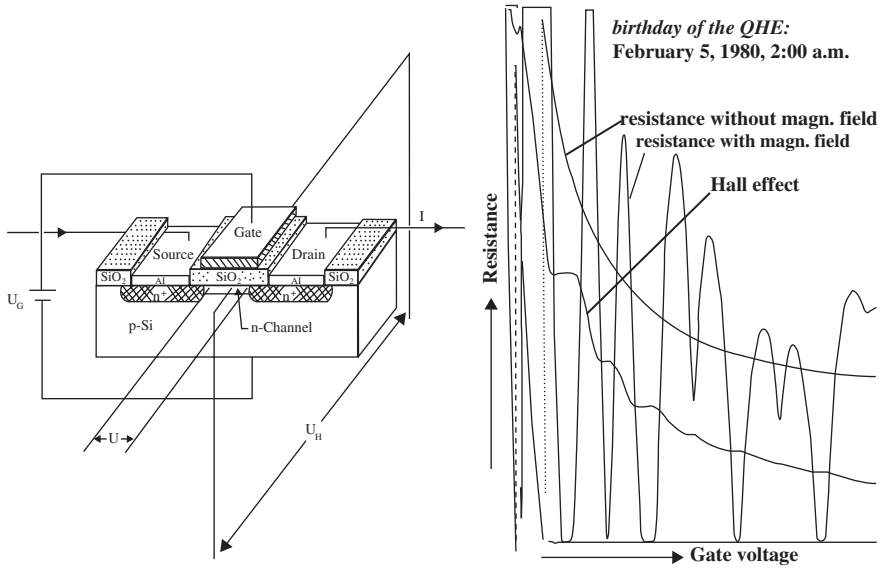
Fig. 7.6 Integer Quantum Hall effect: electrical resistance and Hall resistance in a high magnetic field and at a temperature of 1.5 K, plotted as a function of the gate voltage for the two-dimensional electron gas of the field-effect transistor made from silicon shown on the left, in which early on February 5, 1980 Klaus von Klitzing discovered the quantum Hall effect. The smooth resistance curve without any steps was observed in the absence of a magnetic field. (Klaus von Klitzing)
