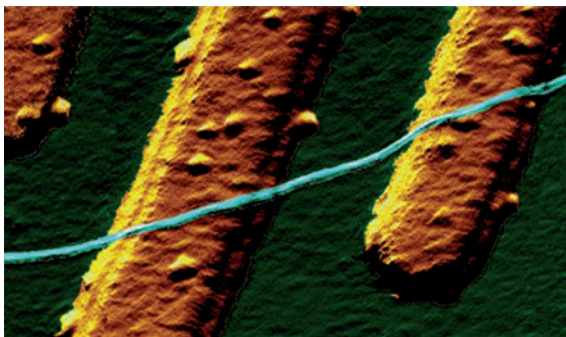
Fig. 11.8 Single-wall carbon nanotube placed between two platinum electrodes. The width of the electrodes is 100 nm. (C. Dekker)
