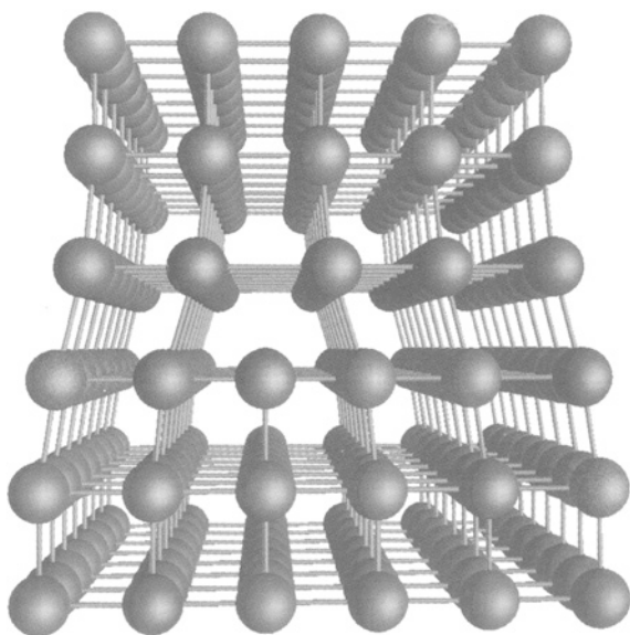
Fig. 12.4 Model of an edge dislocation in a simple-cubic lattice. In the lower half one can see an additional ( vertical ) plane of lattice atoms. (W. Sigle)
