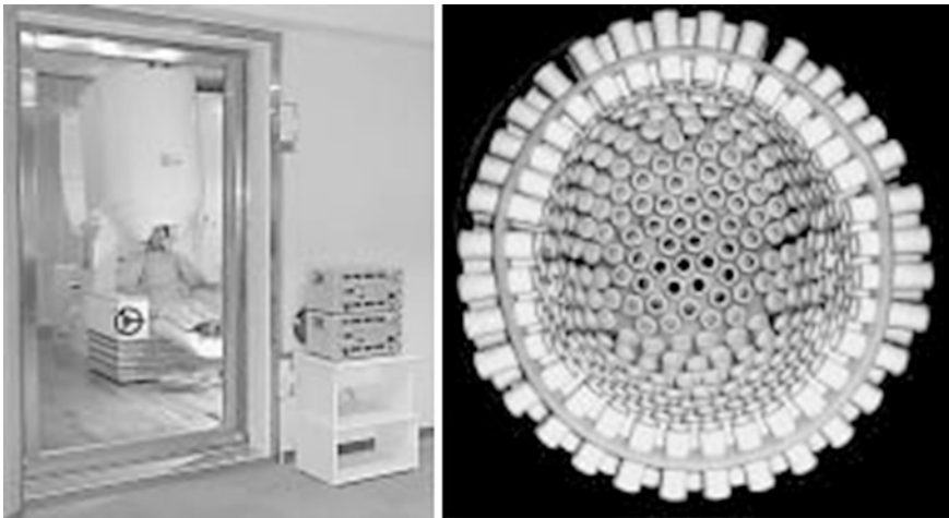
Fig. 8.15 Magneto-encephalography. Left Whole system with the test person carrying the helmet containing the SQUID magnetic-field sensors, within a magnetically shielded chamber. Right View into the helmet having an arrangement of 151 SQUID sensors ( photos MEG International Services Ltd.)
