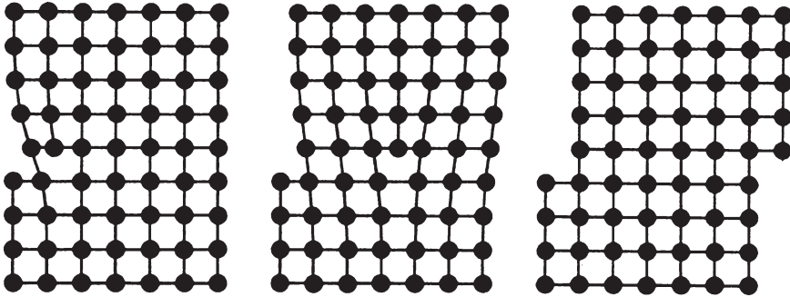
Fig. 12.5 Slippage along a gliding plane, caused by the motion of an edge dislocation, schematically. Left hand The dislocation has been formed at the crystal edge on the left . Middle The dislocation has reached the middle of the crystal. Right hand The dislocation has left the crystal at the edge on the right , and has left behind a slippage step. (U. Essmann)
