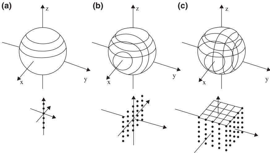
Fig. 2.7 Generation of the Laue diagram as the interference pattern due to the diffraction of X-rays at a three-dimensional point lattice. a For a one-dimensional chain of points, the directions of maximum or minimum intensity lie on cones arranged around the one-dimensional chain. On the surface of an imagined sphere , having its center at the common tip of this family of cones, the directions of maximum or minimum intensity yield a series of circles . b For a two-dimensional planar lattice of points we must add a second family of cones which is arranged around the direction of the second, newly-added straight line of points. Now a second series of circles appears on the surface of the imagined sphere . The points of intersection of these circles then yield the directions of maximum or minimum intensity. c Finally, for a three-dimensional point lattice we deal correspondingly with three families of cones. However, in general the resulting three series of circles on the surface of the imagined sphere no longer have common points of intersection, which mark the directions of maximum or minimum intensity. Now such common points of intersection only exist for special values of the wavelength or frequency of the X-rays
