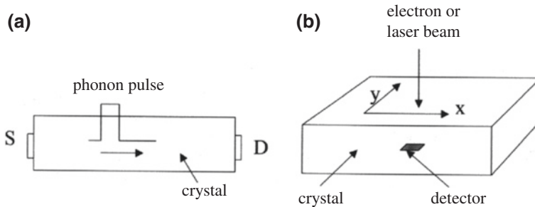
Fig. 3.7 Ballistic propagation of phonons at low temperatures. a Scheme of an experiment to measure the propagation time of the phonons. On the left hand side of the crystal the phonons are generated by means of a heat pulse applied to the source S , and subsequently they are detected on the right hand side of the crystal with the detector D . A thin metal layer deposited on the crystal surface can act as a source by means of the application of an electric current pulse. A deposited thin layer, the electric resistance of which responds sensitively to pulsed temperature changes, can also serve as detector. b A pulsed electron beam or laser beam, directed at the crystal surface at one side of the crystal, can also be used for the generation of a phonon pulse. If furthermore the beam is scanned over the crystal surface, while the detector remains locally fixed on the opposite side of the crystal, the ballistic propagation of the phonons can be studied as a function of the propagation direction in the crystal
