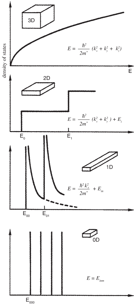
Fig. 7.3 Dependence of the density of states upon the energy E at zero magnetic field in the four cases of a different number of spatial dimensions from three ( top ) to zero ( bottom ). B = 0
