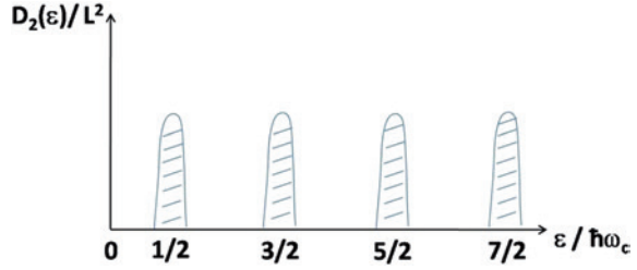
Fig. 7.4 Density of states per area D_2(\epsilon)/L^2 , plotted versus the normalized energy \epsilon/\hbar\omega_c
