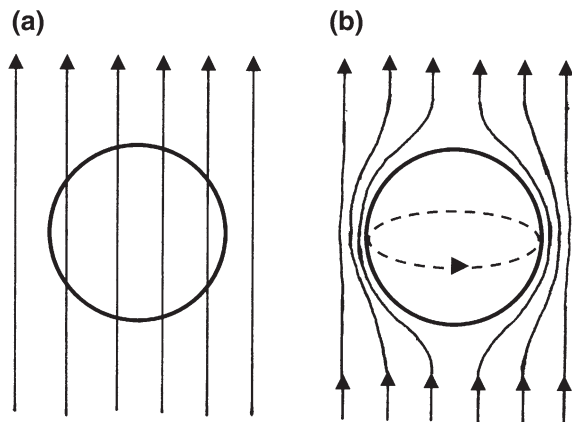
Fig. 8.5 Meissner effect. a In the normal state above its critical temperature, the superconducting sphere is completely penetrated by the external magnetic field. b Below its critical temperature the superconductor completely expels the magnetic field from its interior as long as the critical magnetic field is not exceeded. The field expulsion is accomplished by means of electric currents, flowing without losses on the surface around the superconductor and thereby shielding the interior of the superconductor against the magnetic field
