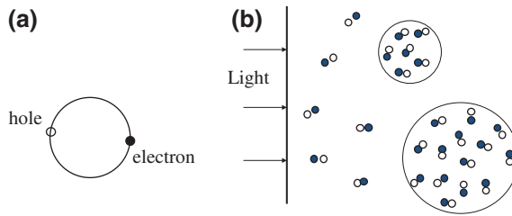
Fig. 6.3 Energetic excitation of an electron from the upper edge of the valence band into the conduction band by means of the absorption of a photon. a An electron-hole pair generated in this way can assume the bound state of an “exciton”. b In a semiconductor crystal, at low temperatures and sufficiently high concentration, the excitons condense into droplets of the electron-hole liquid
