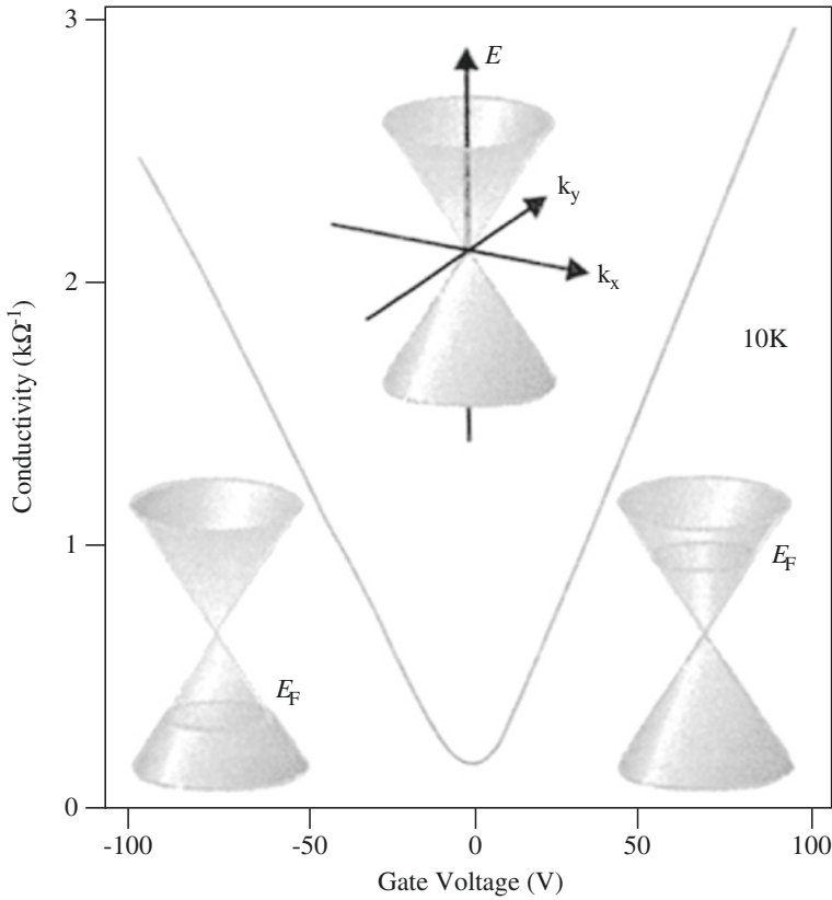
Fig. 11.9 In graphene, the concentration of the charge carriers and the electrical conductivity can be varied strongly, by means of an attached gate electrode and the electric field effect. The figure shows the dependence of the conductivity upon the gate voltage and the linear dependence of the energy E of the electrons upon the wave vector \mathbf{k} , E(\mathbf{k}) , for three values of the Fermi energy E_F , in the case of negative, vanishing, and positive gate voltage (A. Geim)
