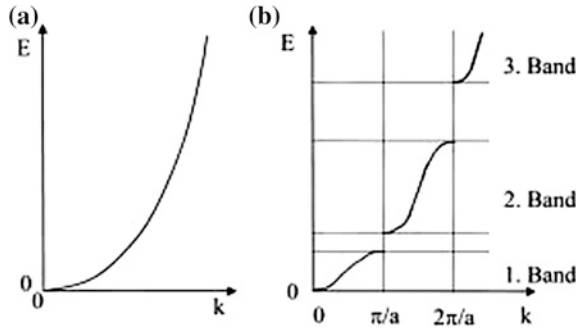
Fig. 4.5 Energy bands in crystals. In the crystal lattice the continuous energy spectrum of free electrons (a) is divided into different energy bands, which are separated from each other by forbidden energy gaps (b). E energy; k wave vector; a distance between neighbors in the crystal lattice
