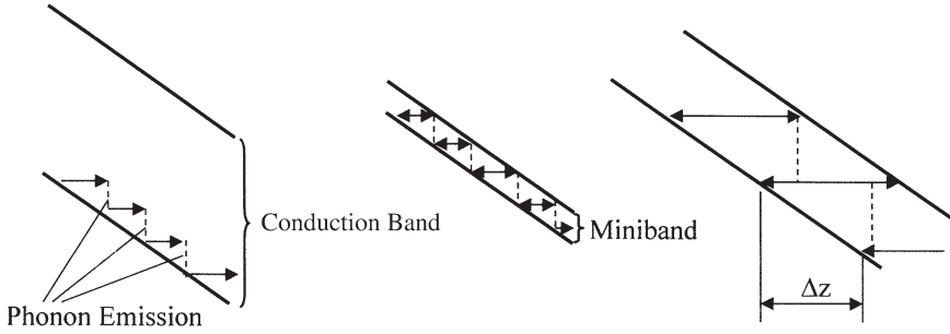
Fig. 11.2 In an electric field, the energy bands are inclined in the field direction because of the potential gradient, and during their motion the electrons are brought closer to the upper edge of the conduction band. However, in a standard semiconductor ( left side ) the electrons already experience a collision process, during which their energy is lowered because of the emission of a phonon, long before they reach the upper edge of the band. On the other hand, in the narrow miniband of a semiconductor superlattice ( middle ) the electrons reach the upper band edge long before a collision process takes place. At the upper band edge they undergo a Bragg reflection, and this process repeats itself as a “Bloch oscillation”, until it is interrupted by a collision process. The enlarged section of a miniband ( right side ) shows how the electrons move by a distance \Delta z in the field direction with each collision process, at which their energy is lowered by the emission of a phonon
