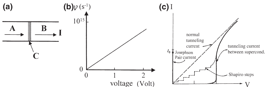
Fig. 8.14 Josephson oscillation of the supercurrent between the superconducting electrodes of a tunnel junction in the presence of an electric voltage across the junction. a In a Josephson junction, the two superconducting electrodes A and B are only weakly coupled to each other, for example, by means of a thin, electrically insulating barrier C, which allows electric current to flow only because of the quantum mechanical tunneling process. b The frequency \nu of the Josephson oscillation of the supercurrent between the two electrodes increases proportionally with the electric voltage V across the junction. At a voltage of 1 V the frequency is about 483,000 GHz. c Electric current I plotted versus the voltage V of a Josephson junction. The solid and the dashed curve show the tunneling current in the case of superconductivity and in the case of normal conductance, respectively. At 0 V we see the Josephson pair current flowing without resistance up to its maximum value I_0 . During irradiation of the junction with microwaves the current-voltage characteristic displays the “Shapiro steps”, which are caused by the combined action of the Josephson oscillation within the junction and the microwaves
