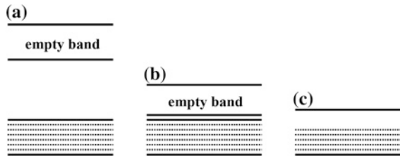
Fig. 4.6 Energy-band model of the electric conductivity of crystals. a A completely filled energy band having a large energy distance to the next higher, but still completely empty energy band, yields an electric insulator. b A completely filled energy band with only a small energy distance to the next higher, but still nearly empty energy band, results in a semiconductor. c A well, but not yet completely filled energy band yields the electric conductance of a metal
