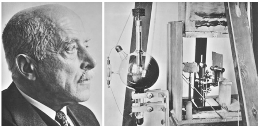
Fig. 2.4 Left Max von Laue. Right set-up of the Laue experiment. On the left we note the X-ray tube and on the right the stage for mounting the crystal ( Photos Deutsches Museum)
