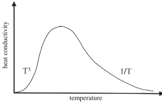
Fig. 3.6 Temperature dependence of the heat conductivity of an electrical insulator (schematically)
