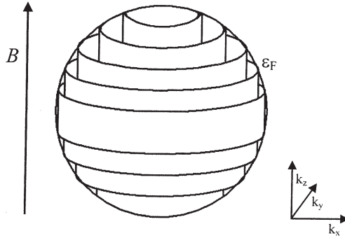
Fig. 7.2 In high magnetic fields the energy quantization according to Landau leads to a redistribution of the states, which can be occupied by the electrons in \mathbf{k} -space, onto the walls of a family of coaxial cylinders. The common axis of the cylinders is oriented along the direction of the magnetic field. The distance between the cylinder walls in \mathbf{k} -space increases proportionally with the magnetic field
