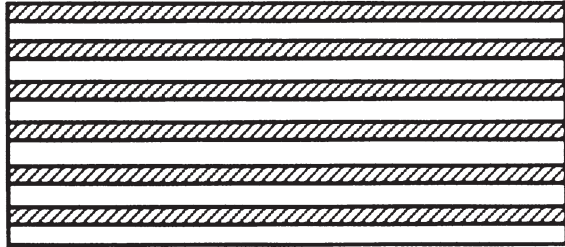
Fig. 11.1 In a superlattice, thin layers of two different metals or semiconductors are alternately stacked on top of each other with high regularity
