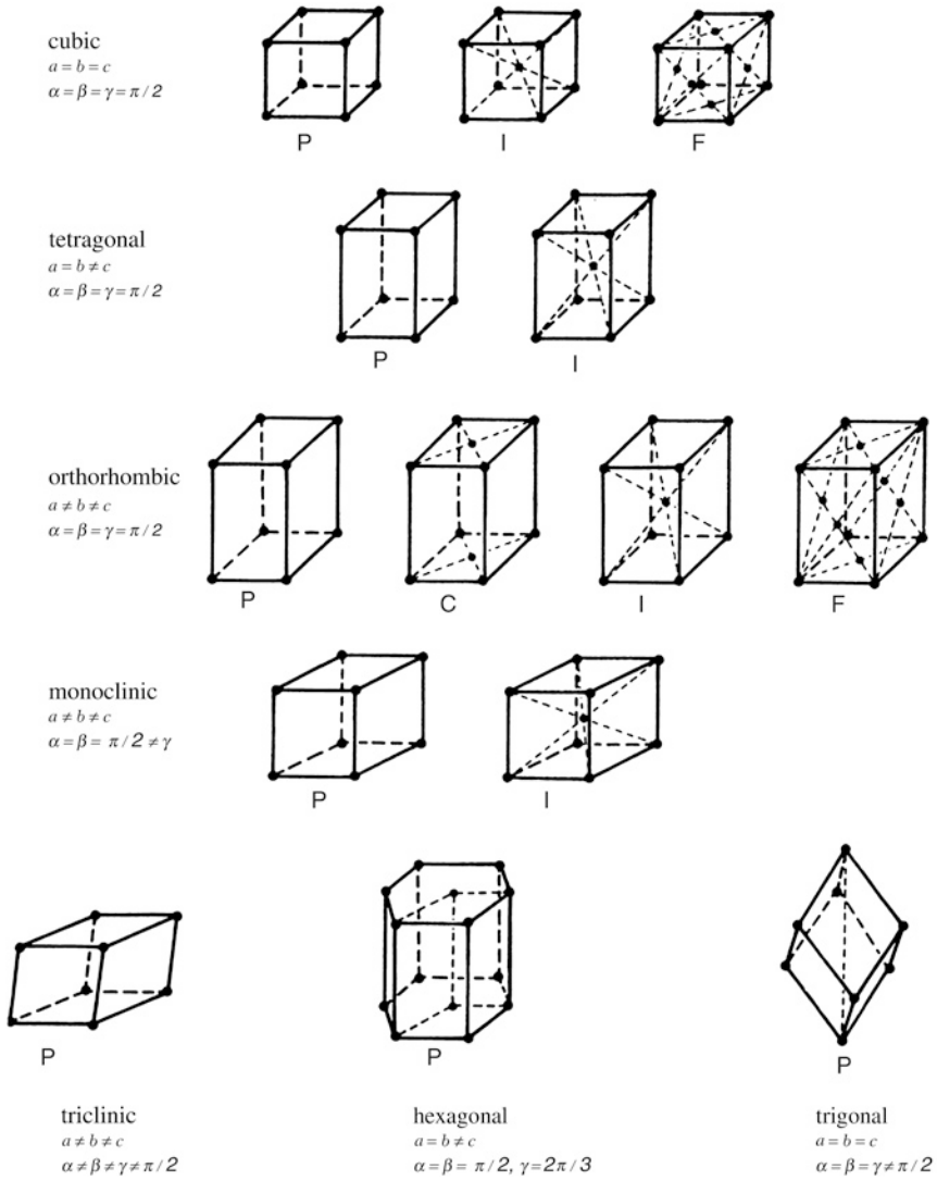
Fig. 2.2 The fourteen Bravais lattices representing all possibilities for the construction of a three-dimensional crystal lattice
