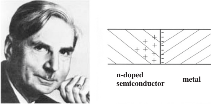
Fig. 6.4 Walter Schottky ( photo Deutsches Museum). Metal-semiconductor contact, also called Schottky contact ( right ). At the junction between an n-doped semiconductor and a metal, within the semiconductor a depletion zone of the mobile electrons is generated, in which the positively ionized donors remain behind. At the adjoining metal surface, negative charges accumulate. In the case of a p-doped semiconductor, negatively ionized acceptors remain behind in the depletion zone
