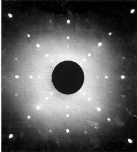
Fig. 2.8 Laue diagram of a cubic \text{K}_2\text{SnCl}_6 crystal obtained by X-ray diffraction (Photo J. Ihlinger)
