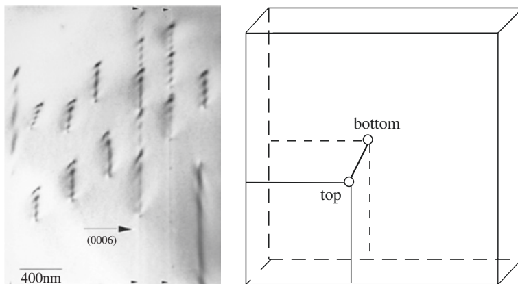
Fig. 12.6 Two-beam image showing several parallel edge dislocations in hexagonal BaTiO 3 ceramics. The dislocations were imaged by diffraction contrast in a transmission electron microscope. Bragg diffracting planes are bent due to the strain field of the dislocations yielding a contrast along the dislocation line. Right sketch of a dislocation penetrating the TEM foil (about 100 nm thick) from top to bottom . (O. Eibl)
