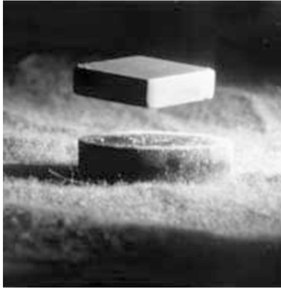
Fig. 8.7 Experimental demonstration of the Meissner effect. A small rectangular piece of a high-temperature superconductor cooled down to the temperature of liquid nitrogen is suspended above a ferromagnetic disk. A repulsive force exists between this ferromagnet and the shielding currents induced in the superconductor because of the Meissner effect ( photo Rainer Straub)
