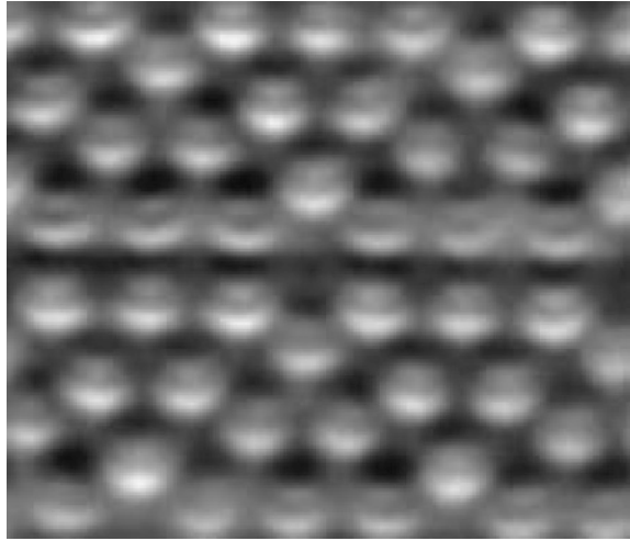
Fig. 1.10 Image of the individual atoms of a section of 5 \text{ nm} \times 5 \text{ nm} area on the surface of a silicon crystal, generated by means of atomic force microscopy. On the silicon atoms we can see a subatomic structure resulting from the electron orbitals ( photo F. J. Giessibl )
