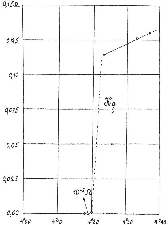
Fig. 8.2 Discovery of superconductivity. Electrical resistance in ohms of a mercury sample plotted as a function of the temperature in Kelvin (H. Kamerlingh Onnes)
