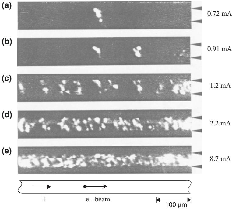
Fig. 9.4 Granular structure of one of the first prepared thin layers of the cuprate superconductor Y_1Ba_2Cu_3O_7 . The layer is 30\ \mu\text{m} wide and runs horizontally. The arrow-heads on the right-hand side mark the upper and the lower edge of the layer, respectively. Bright regions indicate the locations in which electrical resistance appears within the layer during electric current flow. The dark regions are superconducting. From a to e the electric current was increased successively from 0.7 mA at (a) up to 8.7 mA at (e) . The images show the pronounced spatial inhomogeneity of the layer, having large spatial fluctuations of the local critical electric current density. The images were obtained using the method of low-temperature scanning electron microscopy. The temperature was 53 K
