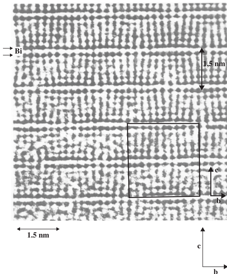
Fig. 9.3 High-resolution electron-microscopic image of the cuprate superconductor \text{Bi}_2\text{Sr}_2\text{CaCu}_2\text{O}_{8+\delta} . The two arrows at the upper left show two rows of bismuth atoms. At the bottom , the direction of the crystallographic b - and c -axis is indicated. The c -axis is oriented perpendicular to the \text{CuO}_2 planes of the cuprate (O. Eibl)
