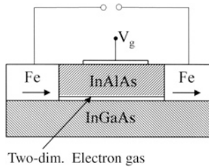
Fig. 10.8 Schematics of a spin-polarized field-effect transistor. The electric current passes through the two-dimensional electron gas at the interface of a semiconductor heterostructure of InGaAs and InAlAs. The current flow is controlled by the voltage V_g applied to the gate electrode
