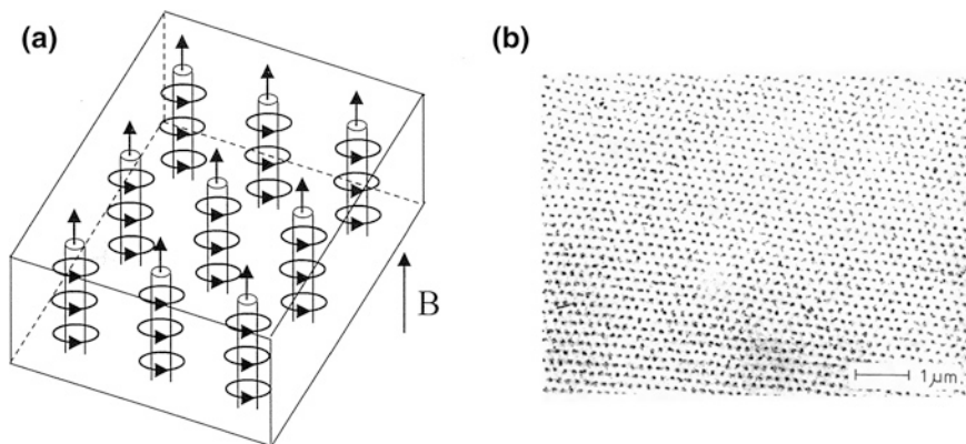
Fig. 8.9 Superconducting mixed state characterized by a lattice of quantized magnetic flux lines, proposed for the first time by Abrikosov. a Schematics. A total of nine magnetic flux lines are shown. Each flux line (like a thread carrying a magnetic field) is surrounded by superconducting circular currents. b Experimental demonstration, by means of the Bitter decoration technique, of the Abrikosov lattice of magnetic flux lines in a plate of superconducting niobium with 0.5 mm thickness. The many dark spots mark the locations at which the individual magnetic flux lines reach the surface of the superconducting plate (U. Essmann)
