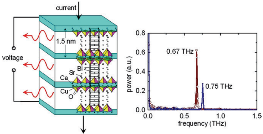
Fig. 9.9 Intrinsic Josephson contact as a source of microwaves. Left Scheme of a staple of three Josephson contacts of a superconducting \text{Bi}_2\text{Sr}_2\text{CaCu}_2\text{O}_8 (BSCCO) crystal. The copper-oxide planes (shown in dark color ) run along the base of the \text{CuO} -pyramids. Right Emitted microwave spectrum of a BSCCO-crystal (R. Kleiner)
