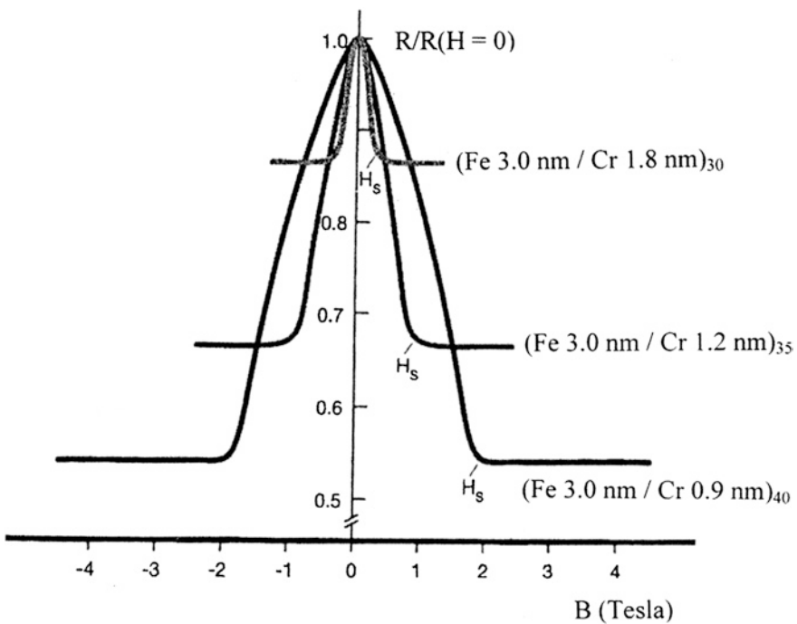
Fig. 10.7 Giant magneto-resistance: Electrical resistance (in units of the resistance at zero magnetic field) plotted as a function of the external magnetic field B for different iron-chromium multi-layers at the temperature of 4.2 K. H_S denotes the magnetic field, at which the magnetizations of the iron layers become oriented in parallel. Identification of the multi-layer structures: for example, (\text{Fe } 3.0 \text{ nm}/\text{Cr } 1.2 \text{ nm})_{35} denotes a multi-layer package consisting of 35 double layers of one 3.0 nm layer of iron and one 1.2 nm layer of chromium (M.N. Baibich)
