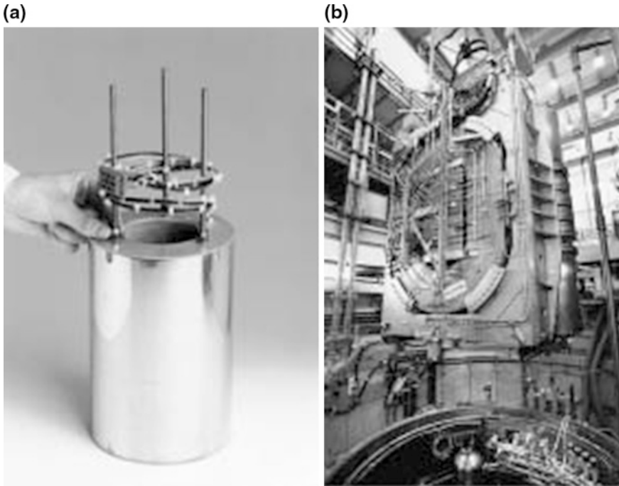
Fig. 8.16 Superconducting magnetic coils. a Commercially available coil for research purposes. The coil is wound from niobium-titanium (NbTi) wire and can generate a magnetic field of up to 9 Tesla, corresponding to about 1 million times the magnetic field of the earth (Oxford). b Superconducting model coil with its test set-up for a toroidal magnetic field during lowering into the cryo-container of an experimental plant at the German Research Center Karlsruhe. The experimental plant serves to develop the technology of magnetic plasma confinement for the nuclear fusion process. The outer dimensions of the oval model coil are 2.55 \times 3.60 \times 0.58 m. During its operation an electric current of 80,000 Ampère is flowing through the coil. The total coil set-up weighs 107 tons and must be cooled down to 4.5 K. The available inner diameter and height of the cryo-container is 4.3 and 6.6 m, respectively (Research Center Karlsruhe KIT)
