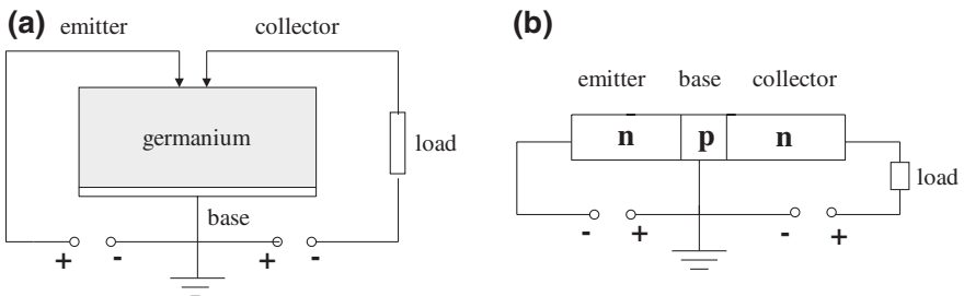
Fig. 6.6 Transistor principle: a Point-contact transistor as it was used originally by Bardeen and Brattain. Two gold contacts are pressed upon an n-doped germanium crystal within a distance from each other of only about 50 \mu\text{m} . On the opposite side of the germanium crystal a third metal contact, the “base”, is attached. One gold contact acts as emitter and injects holes into the germanium crystal. The holes are collected again by the other gold contact, acting as the collector. b Junction transistor according to Shockley. A p-doped semiconductor is placed between two n-doped semiconductors in such a way, that two p-n junctions are formed mirror-symmetrically. Whereas one n-doped semiconductor serves as the emitter, the other n-doped semiconductor acts as the collector. The p-doped region in the center functions as the base
