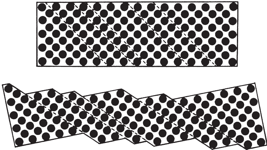
Fig. 12.3 Deformation of a crystal due to slippage, schematically. Only the front plane of the crystal lattice is shown, and additional lattice planes are further behind. The microscopic crystal structure in the undeformed ( top ) and in the deformed state ( bottom ) remains the same. (U. Essmann)
