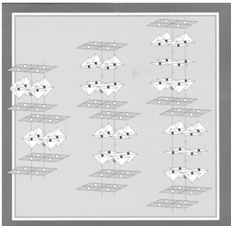
Fig. 9.2 Crystal structure of different cuprate superconductors. At the six corners of the bright octahedrons or at the five corners of the bright pyramids there are oxygen atoms. The centers of the octahedrons, or of the basic square areas of the pyramids, are occupied by copper atoms (IBM)
