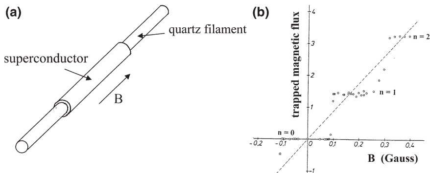
Fig. 8.10 Experimental proof of the magnetic flux quantization in a superconductor. a A tiny superconducting tube with only about 10\ \mu\text{m} diameter is cooled down in the presence of a small magnetic field oriented parallel to the axis of the tube. Below the critical temperature T_C the magnetic field is turned off, and the magnetic flux trapped within the tube is measured. b The frozen-in magnetic flux displays a quantized step structure as a function of the magnetic field B , since only integer multiples of the magnetic flux quantum ( h/2e ) are allowed within the tube. The Figure shows the observation of 0, 1, and 2 magnetic flux quanta, respectively. Without magnetic flux quantization, the data points would fall on the straight dashed line (R. Doll and M. Nábauer)
