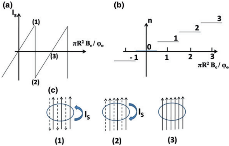
Fig. 8.11 Experimental demonstration of the magnetic flux quantization during entry of magnetic flux into a small superconducting cylinder. a Superconducting shielding current I_s plotted versus the magnetic flux density B_e oriented parallel to the cylinder axis. b Number n of the magnetic flux quanta within the cylinder plotted versus B_e . c Superposition of the applied magnetic field (solid arrows) and of the magnetic field generated by I_s (dashed arrows) at the three points 1–3 from (a). Further details are given in the text
