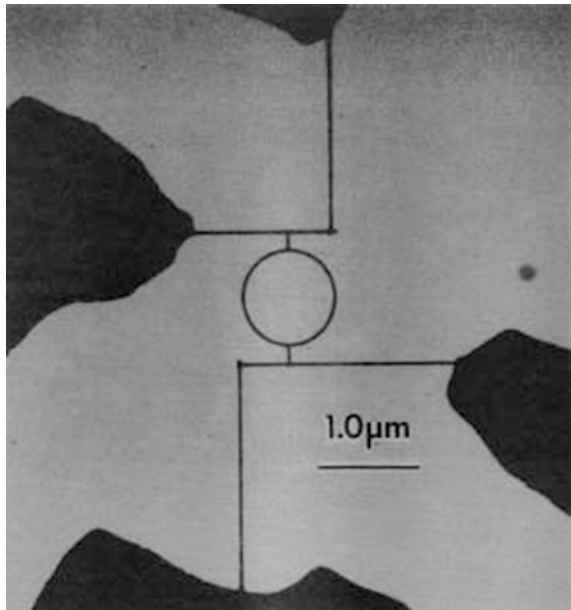
Fig. 11.4 Photograph, produced by an electron-transmission microscope, of a ring fabricated from a gold layer of 38-nm thickness. The inner diameter of the ring is 784 nm. The width of the conducting lines is 41 nm. (R. A. Webb)
