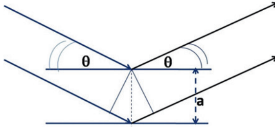
Fig. 2.6 Reflection of a wave at two neighboring lattice planes placed at the distance a . The difference of the distance covered by the wave upon the reflection at the two planes amounts to 2 a \sin \theta . \theta is the angle between the lattice planes and the incoming and the outgoing wave, respectively
