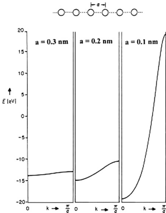
Fig. 4.3 Electronic band structure of a one-dimensional straight chain of hydrogen atoms with a distance between neighbors of 0.3, 0.2, and 0.1 nm, respectively. The electron energy \epsilon is plotted as a function of the wave vector k . For a single isolated hydrogen atom the electron energy is -13.6 eV. The broadening of this energy level results in the energy bands. The energy width of these bands increases strongly with decreasing distance between neighboring atoms (R. Hoffmann)
