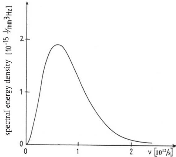
Fig. 3.4 Spectral energy density of the phonons in a germanium crystal at the temperature of 10 K according to the Planck radiation law, plotted versus the phonon frequency \nu
