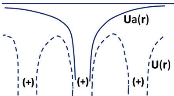
Fig. 4.2 Comparison of the energy of an electron, U_a(\mathbf{r}) , in the case of an isolated individual atom (solid line), and the case of the presence of atoms at the neighboring lattice sites, U(\mathbf{r}) (dashed curve)
