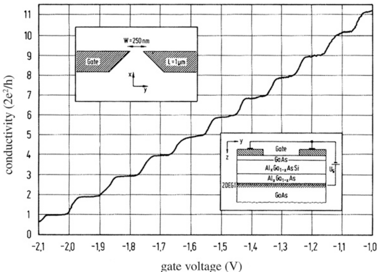
Fig. 11.6 Electrical conductance of a narrow one-dimensional channel in a GaAs/ \text{Al}_x\text{Ga}_{1-x}\text{As} —heterostructure in the quantized unit ( 2e^2/h ) plotted as a function of the gate voltage at a temperature of about 1 K. Inset on upper left arrangement of the gate electrodes on the surface of the heterostructure. Inset on lower right cut through the heterostructure (2DEG two-dimensional electron gas; U_G gate voltage) (B. J. van Wees)
