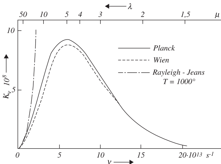
Fig. 3.1 The radiation laws of the black body according to Planck, Wien, as well as Rayleigh and Jeans. Spectral radiation intensity plotted versus the frequency
