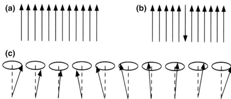
Fig. 10.5 Elementary magnets in a simple ferromagnet. a In the ground state all elementary magnets are oriented in the same direction. b A possible excitation from the ground state: one spin is flipped over. c Spin wave in a chain of spins in a perspective presentation
