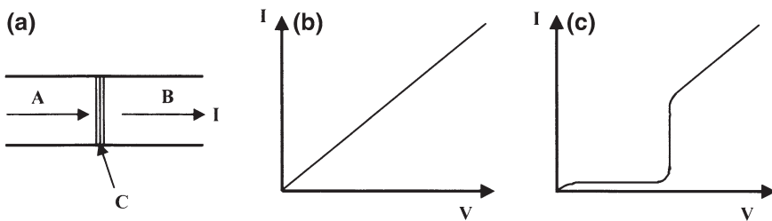
Fig. 8.13 Experimental proof of the energy gap in a superconductor by means of the tunneling experiment of Giaever. a A superconducting electrode A and a normal electrode B are separated from each other by a thin, electrically insulating barrier C, such that the electric current flow across the barrier is only possible because of the quantum mechanical tunneling process. b Electric current I plotted versus the voltage V in the case when both electrodes are metals in the normal state. c Electric current I plotted versus the voltage V in the case when one metal electrode is superconducting. The electric current can start to flow only when the electrical potential difference between the two electrodes has reached the value of the energy gap
