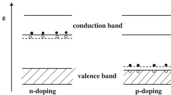
Fig. 6.2 Doped semiconductors. The conduction band is separated from the valence band by a relatively large energy gap. With n-doping, electrons are thermally excited from the donors up to the lower edge of the conduction band. With p-doping, the thermal excitation of the electrons occurs from the upper edge of the valence band up to the energy levels of the acceptors, such that holes remain in the valence band
