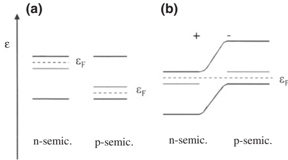
Fig. 6.5 p-n junction. a As long as there exists no connection between the n-doped and the p-doped semiconductor, the energy diagram displays clearly different values of the Fermi energy \epsilon_F in the two semiconductors. b With an electric contact between the n-doped and the p-doped semiconductor, the concentration gradient of the electrons and of the holes between both sides of the junction is equalized by means of diffusion of both kinds of charge carriers to the opposite side, respectively. During this process, positive or negative space-charge regions are generated on both sides of the junction, resulting in a local electric field between both sides. The diffusion process ends when the Fermi energy \epsilon_F has reached the same value on both sides of the junction
