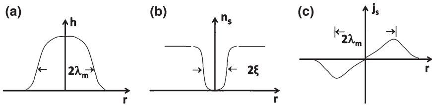
Fig. 8.12 Structure of a single flux line. Local magnetic field h , density of the superconducting electrons n_s , and the circulating superconducting current density j_s as a function of the distance r from the axis of the flux line
