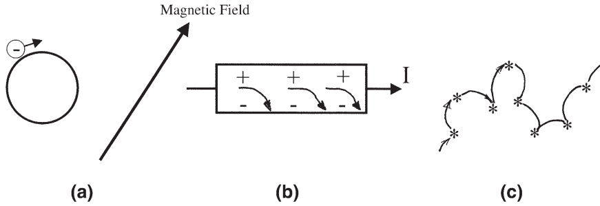
Fig. 7.1 Lorentz force acting on electric charges moving in a magnetic field. The magnetic field is directed perpendicular to the plane of the paper. a Because of the Lorentz force, the motion of electric charges perpendicular to the direction of the magnetic field is deflected onto a circular orbit. b Hall effect: During electric current flow in a conductor, the sideways deflection of the current due to the Lorentz force causes the accumulation of charges with opposite sign, respectively, on both sides of the conductor (assuming that the opposite charges move in the same direction). This results in an electric voltage perpendicular to the main current direction and perpendicular to the direction of the magnetic field. c Magneto-resistance: The deflection of the electric charges into circular orbits because of the Lorentz force hinders the electric current flow along its main direction and causes an increase in the electrical resistance. The crosses mark the locations, where the electrons experience a collision process
