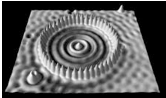
Fig. 1.11 The picture shows a ring of iron atoms placed on a copper surface. In this way an artificial coral reef consisting of 48 iron atoms has been created on an atomic scale. The circular lines appearing within the ring are due the density of the electrons existing within the ring ( photo Almaden Research Center 2000 )
