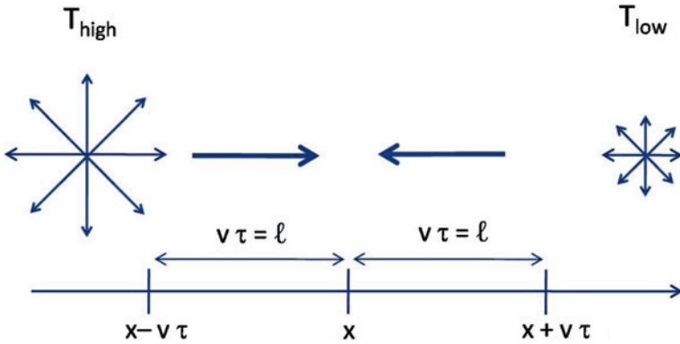
Fig. 5.1 Illustration regarding the heat current density of (5.5). The arrows near T_{\text{high}} and T_{\text{low}} indicate the average electron energy
