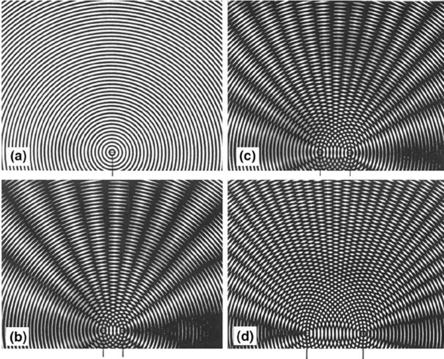
Fig. 2.5 a Propagation of a spherical wave originating from a point. The dark rings illustrate the peaks of the wave which follow each other within the spatial distance of one wavelength. The picture corresponds to a snapshot and shows the wave propagation within a plane as, for example, on a water surface. b Interference between two waves such as shown in (a) , originating from two different centers. From b to d the distance between the two centers increases. In specific directions the peaks and the valleys of the waves coincide, such that both waves annihilate each other. The positions at which the annihilation takes place, appear closer and closer as the distance between the two centers increase
