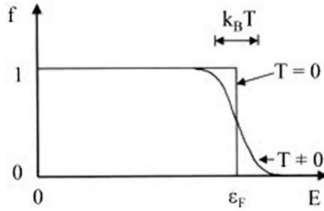
Fig. 5.2 Fermi distribution function: because of the Pauli exclusion principle each quantum mechanical state in a crystal can be occupied at most by only one electron. At the temperature of zero Kelvin, for all energies up to the Fermi energy \epsilon_F the Fermi distribution function has the value of one, and at \epsilon_F it drops abruptly from one to zero. At a finite temperature T , the drop of the Fermi distribution function from one to zero is smeared out along the energy axis, and it occurs at the Fermi energy within an energy width of about k_B T
