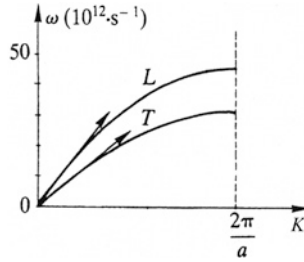
Fig. 3.5 Phonon angular frequency \omega = 2\pi\nu plotted as a function of the wave number K of the phonons (“dispersion curves”) of a copper crystal. The wave vector is oriented along the direction of the cube edges of the cubic unit cell of the crystal. L denotes the longitudinal and T the transverse phonon branch. a = 0.361 nm is the distance between neighbors in the cubic crystal lattice of copper (B.N. Brockhouse)
