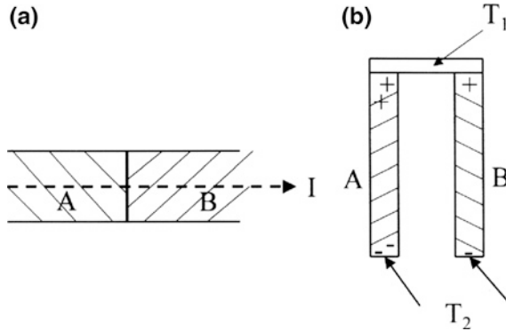
Fig. 5.6 a Peltier effect: if the electric current I passes through the contact zone between two different metals A and B, having a different value of the heat current carried by the same electric current, heating or cooling of the contact zone results, depending upon the current direction. b Seebeck effect: in the temperature gradient between the higher temperature T_1 ( upper side ) and the lower temperature T_2 ( lower side ) in an electrical conductor the mobile electrons are transported from the hot to the cold end of the conductor by means of thermal diffusion. Therefore, at both ends of the conductor, electric charges of opposite sign, respectively, accumulate. The direction of this thermal diffusion process is determined by the details of the Fermi surface and of the collision processes of the electrons. The figure shows two different metals A and B, which are soldered together at the end with the higher temperature. The difference in the thermal diffusion between the two metals results in an electric voltage, the “thermoelectric voltage”, between the lower ends of the two metals
