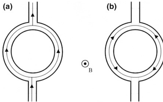
Fig. 11.10 Aharonov-Bohm effect in ring geometry. The external magnetic field is oriented perpendicular to the plane of the ring. a The interference between the trajectories through the right and through the left -half of the ring leads to oscillations in the electrical resistance with periodicity ( h/e ) of the magnetic flux enclosed by the ring. b For a complete revolution of two trajectories around the ring in opposite directions, respectively, the interference results in oscillations of the resistance with periodicity ( h/2e )
