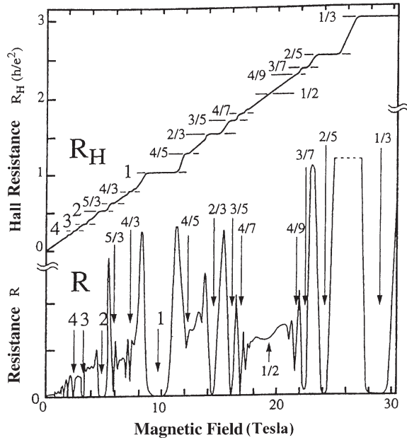
Fig. 7.7 Fractional quantum Hall effect in the two-dimensional electron gas of a modulation doped GaAs/AlGaAs semiconductor hetero-structure at a temperature of about 0.1 K. The electrical resistance R and the Hall Resistance R_H are plotted as a function of the magnetic field. The Hall resistance displays many plateaus for the indicated fractional values of z , if the quantized Hall resistance is written in the form (1/z)(h/e^2) . (Horst L. Störmer)
