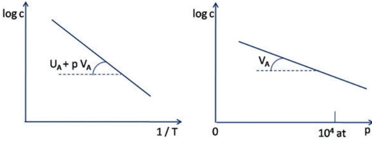
Fig. 12.1 Plot of \log c versus 1/T (left) and versus p (right), schematically after (12.6)
