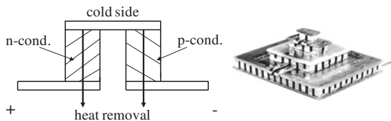
Fig. 6.11 Peltier cooling. Left Schematics of a Peltier cooling device consisting of an n-doped and a p-doped semiconductor. The electric current flows from the left to the right side. Right Commercially available four-stage Peltier cascade. In the individual stages the Peltier legs are clearly visible. With the cascade shown, the temperature can be lowered from room temperature at the warm end down by about 140 K lower than room temperature at the cold end. The lateral dimensions are: lowest stage: 24.0 mm \times 20.6 mm; uppermost stage: 4.5 mm \times 2.4 mm. Total height: 13.6 mm. ( photo KRYOTHERM)
