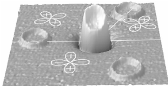
Fig. 9.8 Tricrystal experiment of Tsuei and coworkers for proving the d-wave symmetry of the quantum mechanical wave function of Cooper pairs in the cuprate superconductor \text{Y}_1\text{Ba}_2\text{Cu}_3\text{O}_7 . The substrate is an artificially prepared tricrystal, in which three differently oriented single-crystalline parts of the crystal are separated from each other by atomically sharp grain boundaries. This crystalline structure, including its grain boundaries, is exactly transferred to the superconducting layer prepared on top. The grain boundaries are marked by straight white lines . Within the three crystal parts, separated from each other by the grain boundaries, the differently oriented d-wave symmetry pattern of the Cooper pair wave function is indicated by the diagrams with the four lobes. At different locations, a total of four superconducting rings are fabricated from the YBaCuO layer, whereas the remaining part of the layer is removed. The orientations of the three crystal parts are chosen such that, in the presence of d-wave symmetry of the wave function, within the ring around the common meeting point of the three crystal parts, an exactly half-integer magnetic flux quantum is spontaneously generated, whereas nothing happens at the three other rings. The image was obtained by means of a SQUID scanning microscope, and it clearly shows the half-integer magnetic flux quantum for the ring in the middle around the common meeting point of the three crystal parts. The other rings are only weakly visible (C.C. Tsuei)
