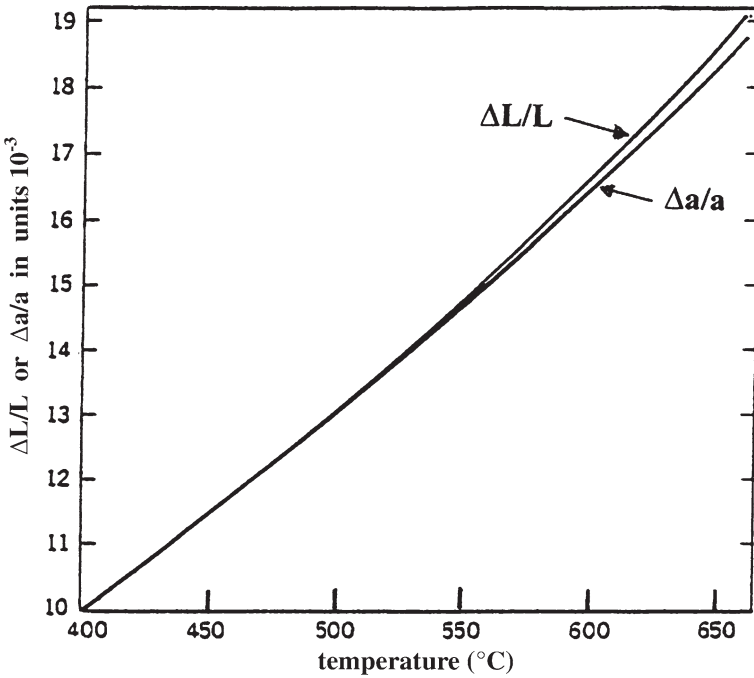
Fig. 12.2 Influence of the vacancies, existing in equilibrium within the crystal lattice, upon the temperature dependence of the crystal volume of aluminum. Because of the thermally generated vacancies, the temperature dependence of the relative length change, \Delta L/L , (upper curve) is slightly larger than the temperature dependence of the relative change of the distance between neighbors in the crystal lattice, \Delta a/a (lower curve). The difference between both curves increases with increasing temperature. (R.O. Simmons and R.W. Balluffi)
