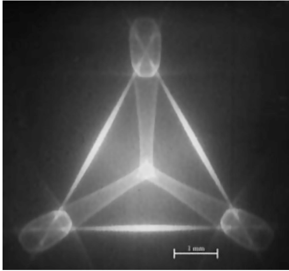
Fig. 3.8 Image of the intensity of the ballistic phonons in dependence on the propagation direction in a silicon single crystal at a temperature of 2.0 K (“phonon imaging”). While the crystal surface on one side is scanned with the electron beam, the intensity of the ballistic phonons is recorded on the opposite side of the crystal with a locally fixed detector in dependence on the coordinate point of the scanned crystal surface. Bright regions correspond to high intensity. The spatially diagonal line of the cubic unit cell of the crystal is oriented perpendicular to the scanned surface of the crystal
