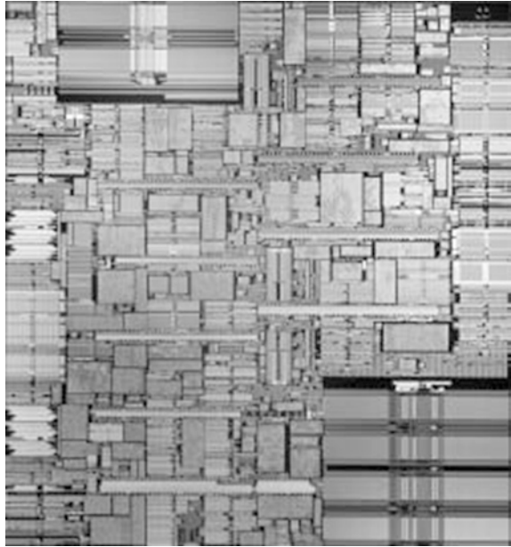
Fig. 6.10 Modern microprocessor chip with the dimensions 12.6 mm \times 12.6 mm. (Here the microprocessor Power 3). There are about 15 million transistors on this chip. (IBM)
