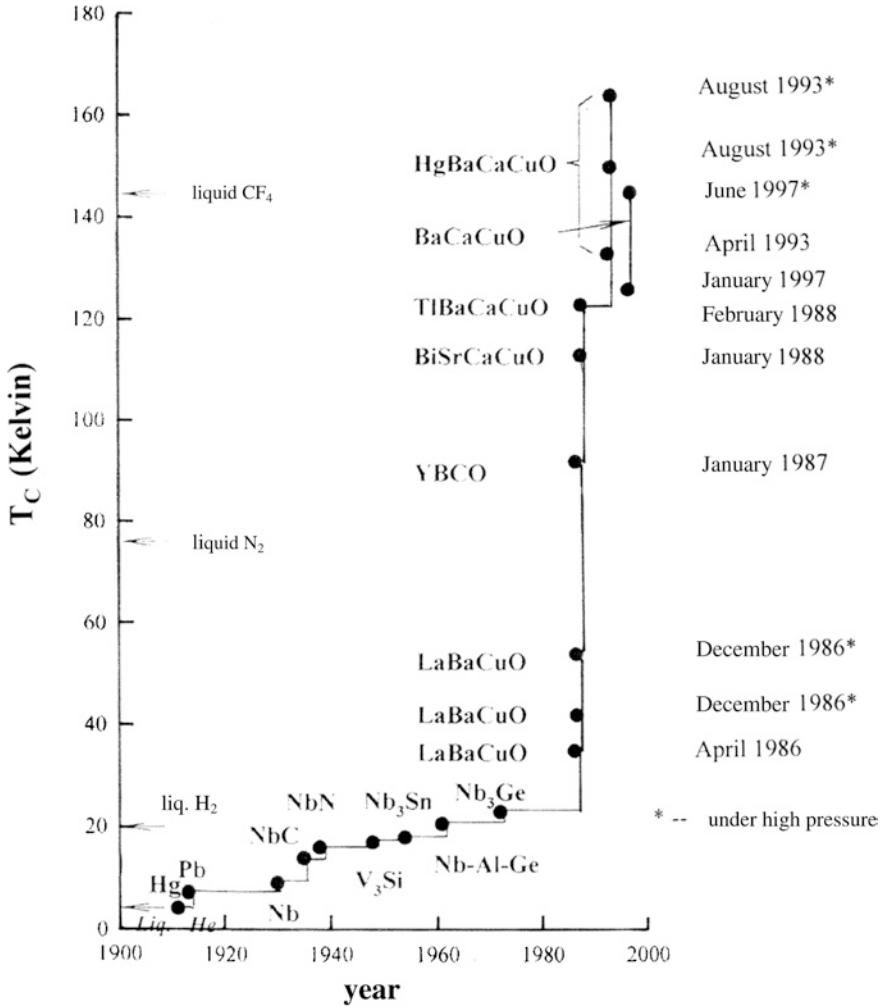
Fig. 9.1 Critical temperature T_c plotted versus the year of discovery of different superconductors. The steep branch of the curve on the right-hand side shows the different high-temperature superconductors. The entries marked with an asterisk indicate where the critical temperature could be increased further under high pressure (C.W. Chu)
